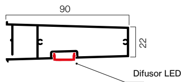
Lama V-90 LED 050531
